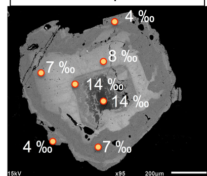
\delta^{18}\text{O} in garnet crystal from a metaquartzite
